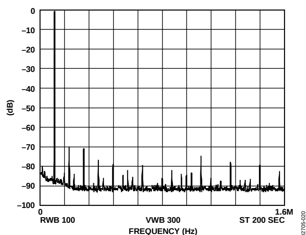
Figure 22. f_{MCLK} = 50 \text{ MHz} ; f_{OUT} = 120 \text{ kHz} , Frequency Word = 009D496
