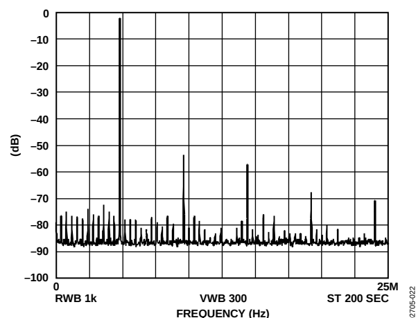
Figure 24. f_{MCLK} = 50 \text{ MHz} ; f_{OUT} = 4.8 \text{ MHz} , Frequency Word = 189374C
