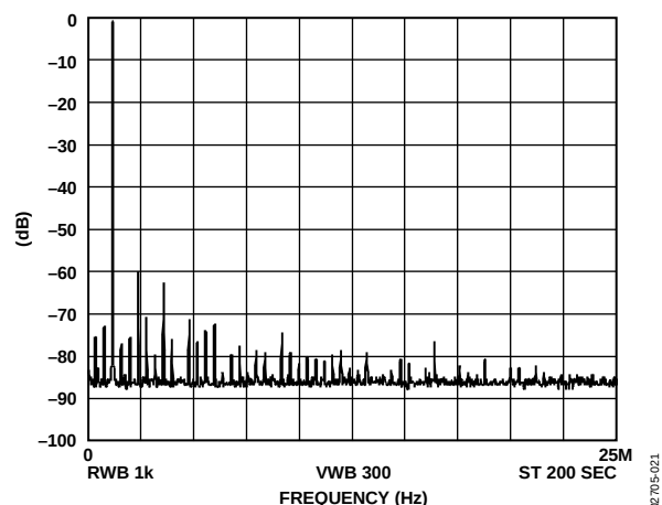
Figure 23. f_{MCLK} = 50 \text{ MHz} ; f_{OUT} = 1.2 \text{ MHz} , Frequency Word = 0624DD3
