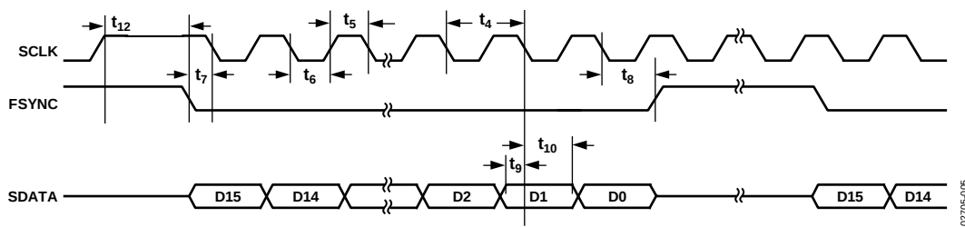
Figure 5. Serial Timing
