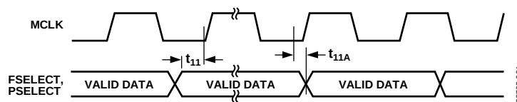
Figure 4. Control Timing
