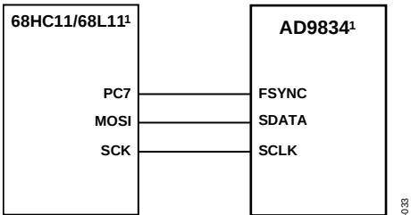
Figure 36. 68HC11/68L11 to AD9834 Interface
